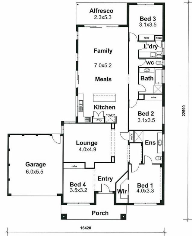
Oakland 200E Area: 250 m 2 (26.91 sq) Minimum width of site required 17.80m. Conditions apply. Optimum 5 star siting to be confirmed.
