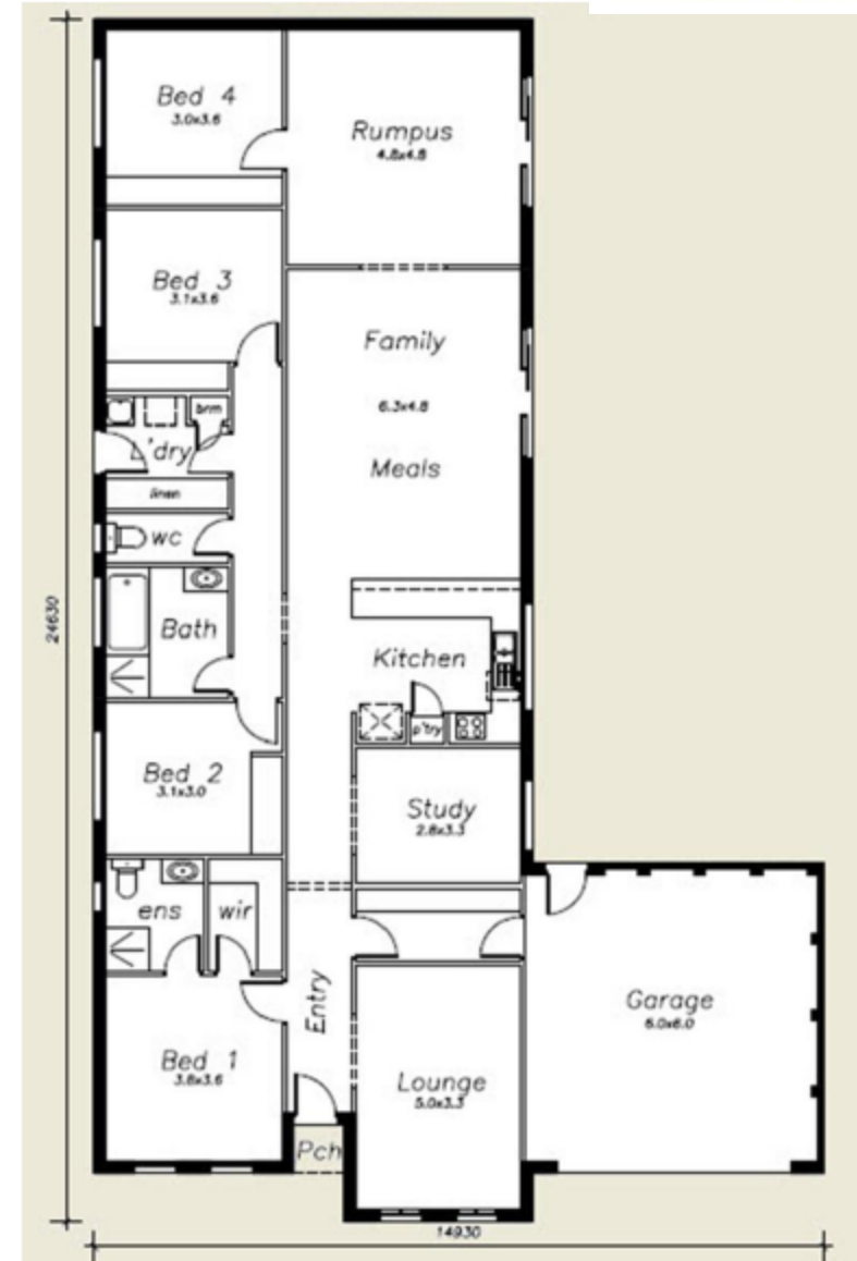
Harmony 240E Area: 251 m2 (27 sq)
