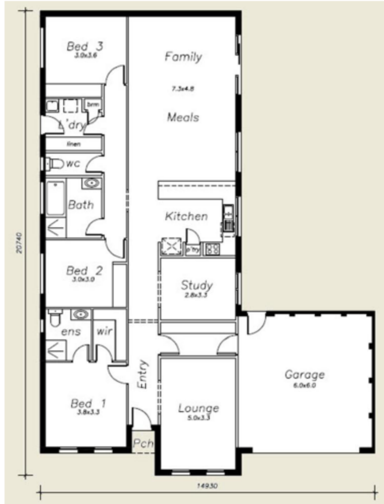
Harmony 190E Area: 213.9 m2 (23 sq)
